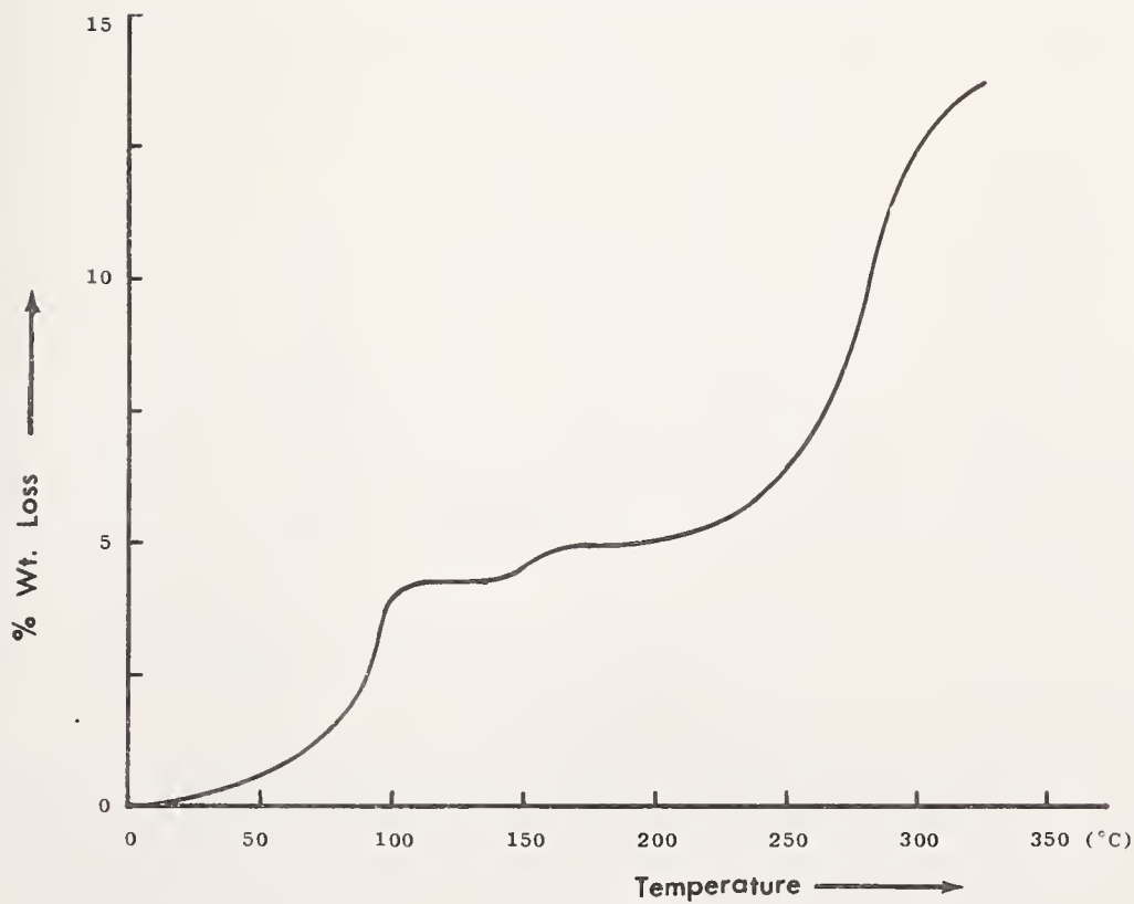
Fig. 3: Percent weight loss of C-10/T-30 prepreg as a function of temperature
